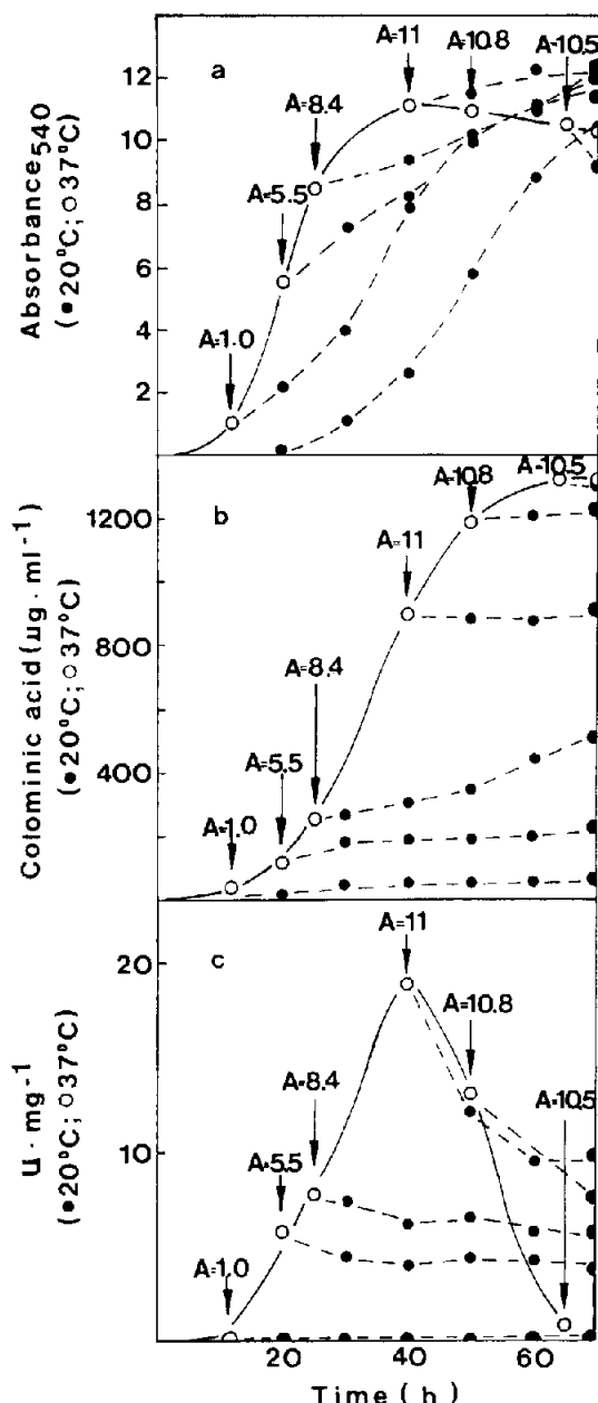
Fig.3. Effect of temperature for transfer of E. coli cultures from 37°C (○) to 20°C (●) on: (a) bacterial growth, (b) colomonic acid production, (c) CMP-Neu5Ac synthetase activity. Arrows indicate the time of transfer. A, absorbance 540 nm.
